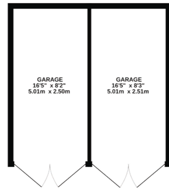
270 sq.ft. (25.1 sq.m.) approx.
